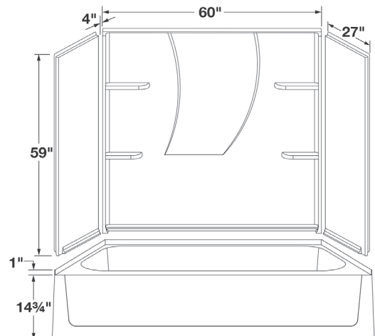
Fits 30"x60" TOPAZ™ Bathtub
